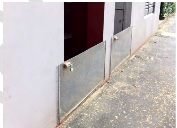
Photo 20: Examples of flood barriers located at commercial premises on Victoria Street.
